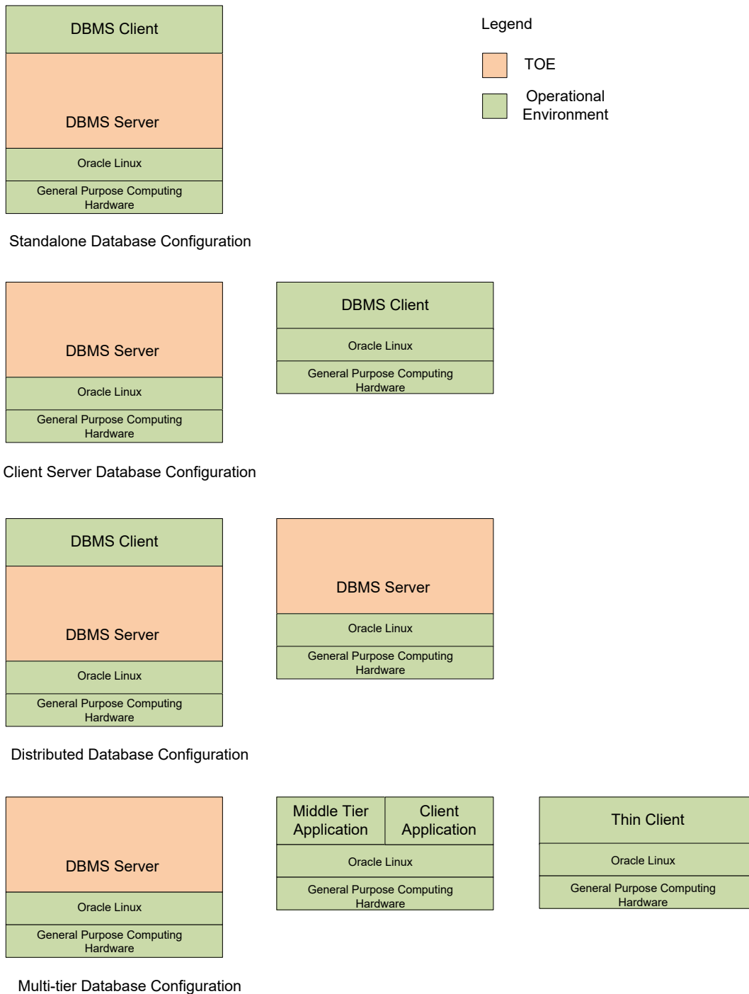
Figure 1 – Oracle Database 19c Diagram
