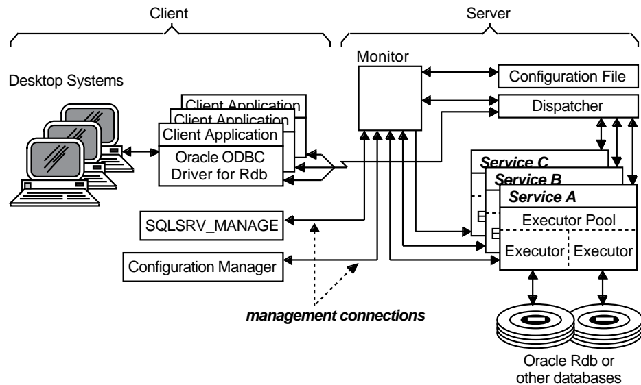
Figure 2–2 Oracle SQL/Services Architecture
