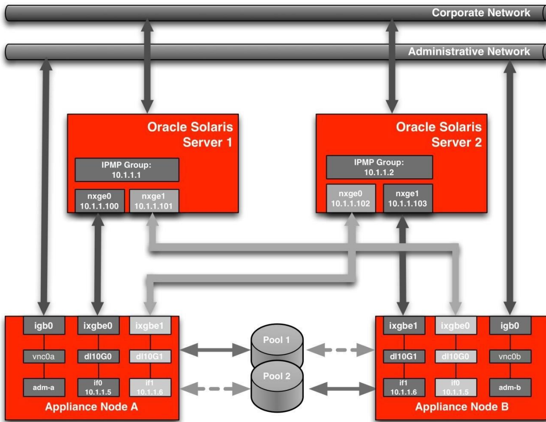
Figure 18. Direct 10 GbE connections
