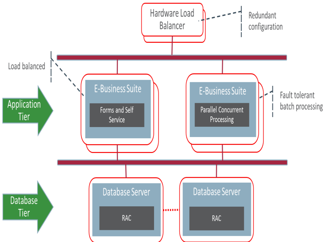
Figure 3 Oracle E-Business Suite High Availability Architecture
