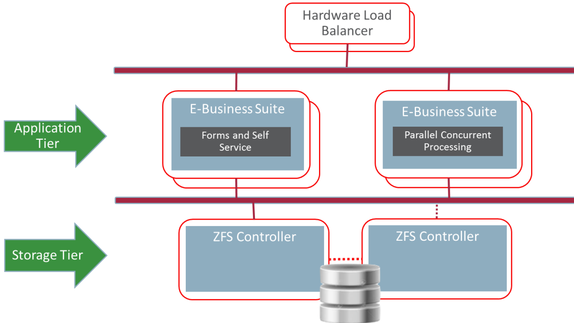
Figure 6 Two application tiers and ZFS filer
