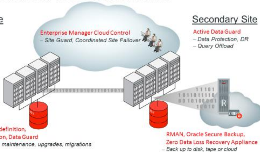
Figure 2 Oracle Database Maximum Availability Architecture
