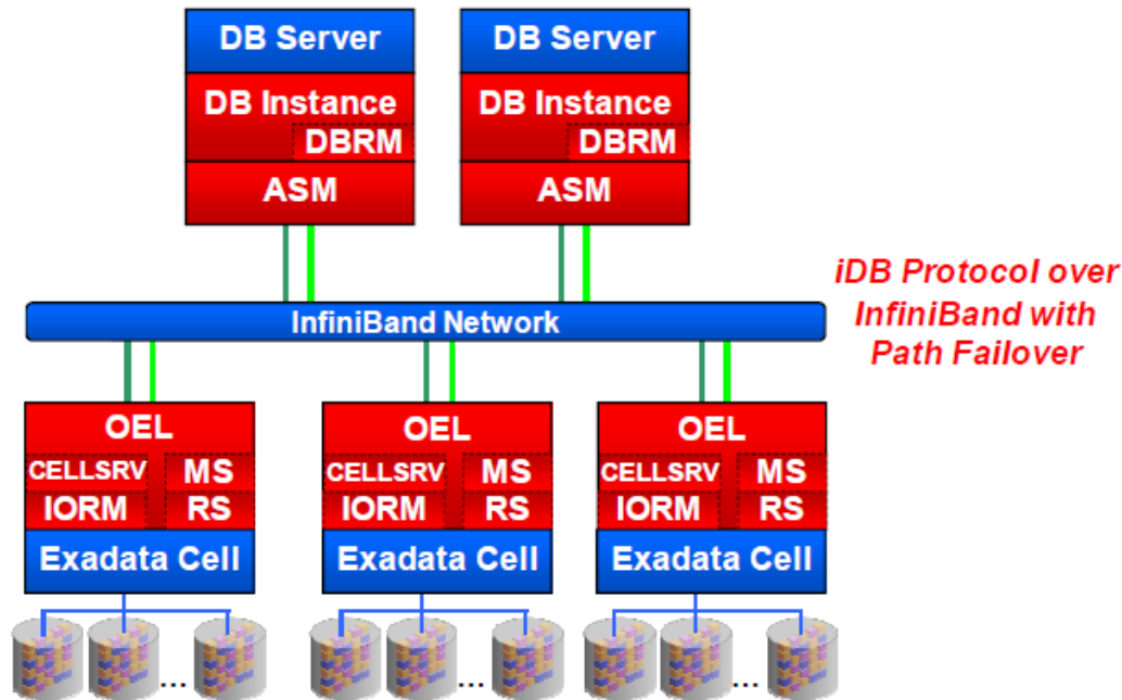
Figure 7 Block diagram showing the hardware and software layout of an Exadata quarter rack
