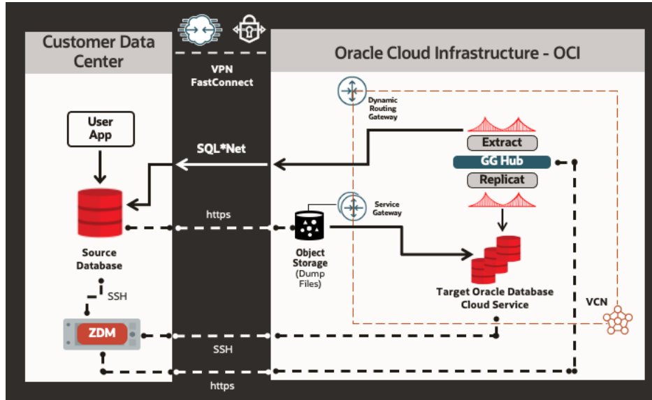
Figure 3. ZDM Logical Online Migration Architectural Diagram
