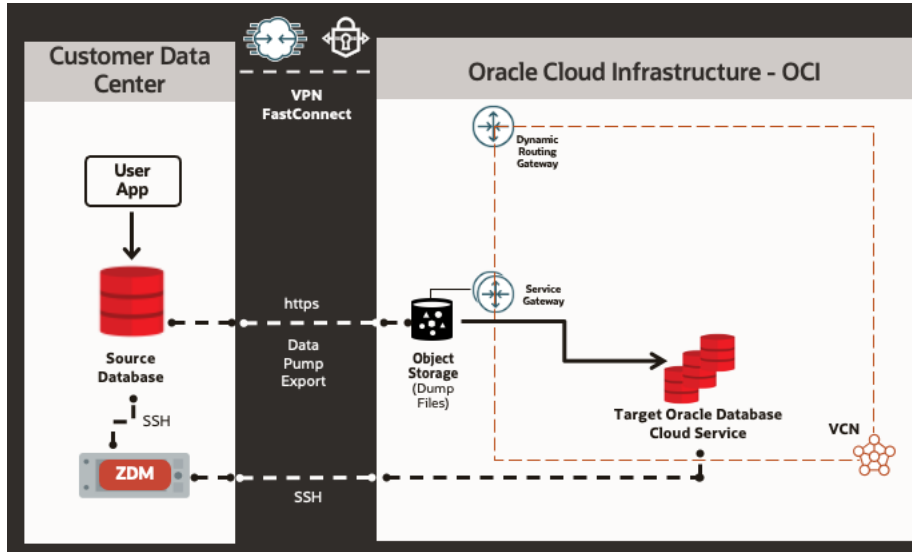
Figure 2. ZDM Logical Offline Migration Architectural Diagram
