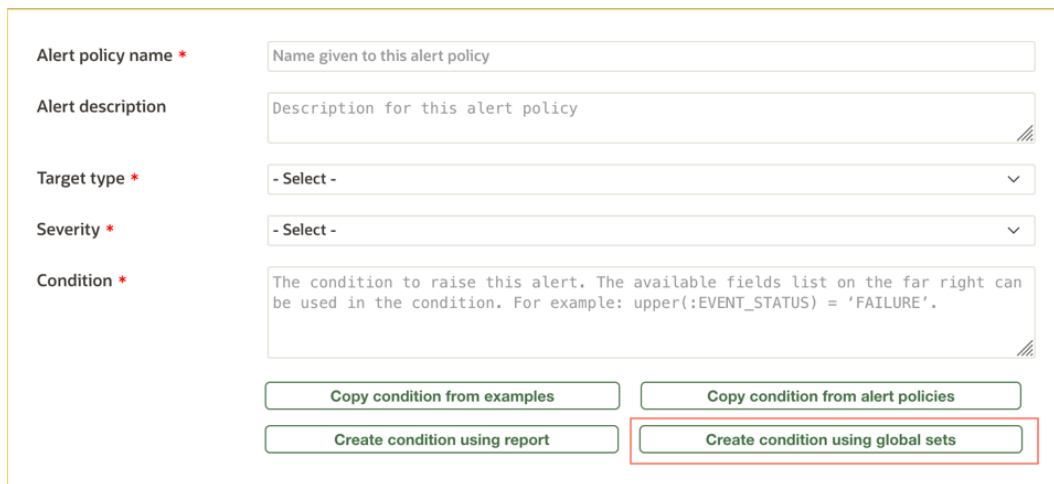
Figure 7. Creating an Alert Policy
