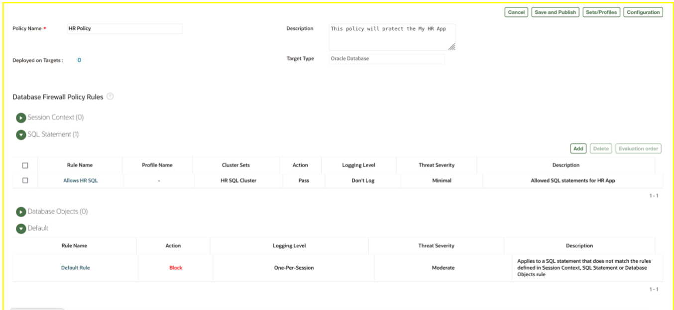
Figure 9. Database Firewall Policies
