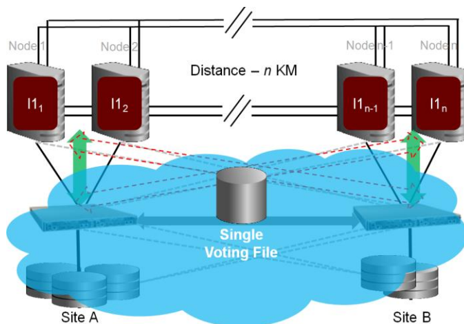
Figure 15: Single Voting File used on Storage Cluster
