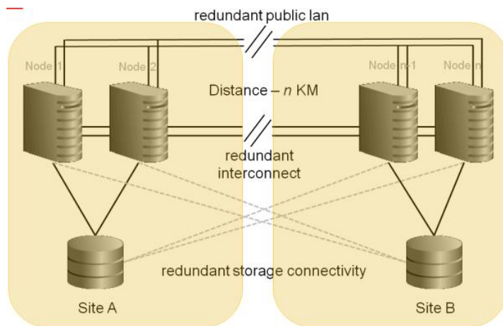
Figure 10: Overall Network Design
