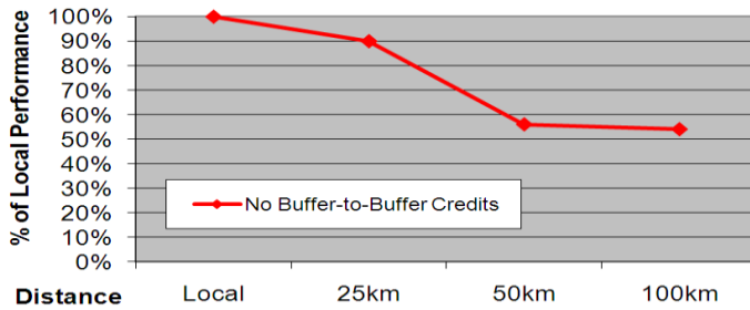
Figure 9: Untuned example – “overall performance impact on applications due to distance”
