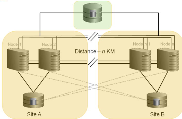
Figure 14: Extended Distance Cluster with Quorum File / Voting File in Third Location
