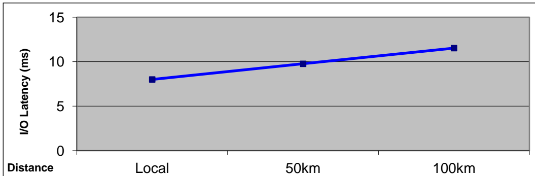
Figure 6: I/O latency increase in ms over distance
