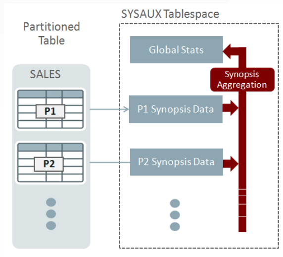
Figure 12: Incremental statistics gathering on a range partitioned table.
