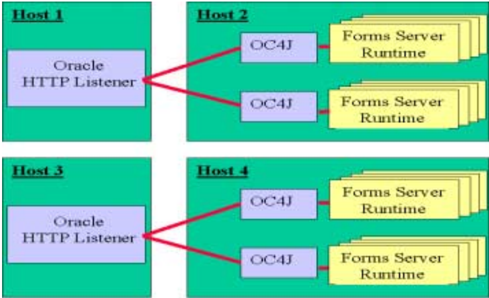
Figure 4-3 Case 3: Multiple OC4J engines and multiple Oracle HTTP Listeners on different hosts.
