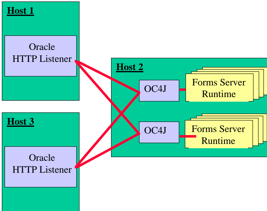
Figure 4-4 Case 4: Multiple Oracle HTTP Listeners on different hosts with multiple OC4J engines on one host
