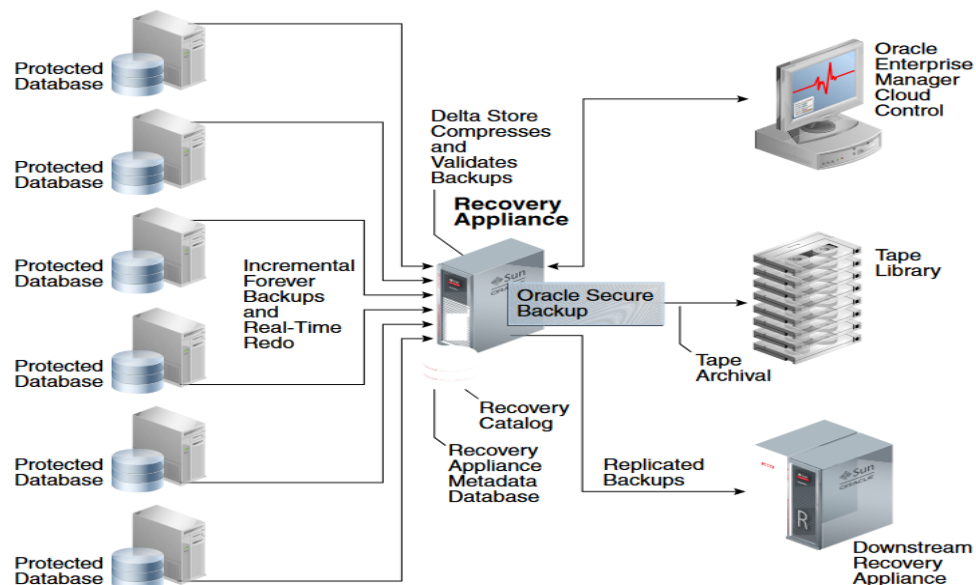
FIGURE 2: Recovery Appliance Architecture and Protected Databases
