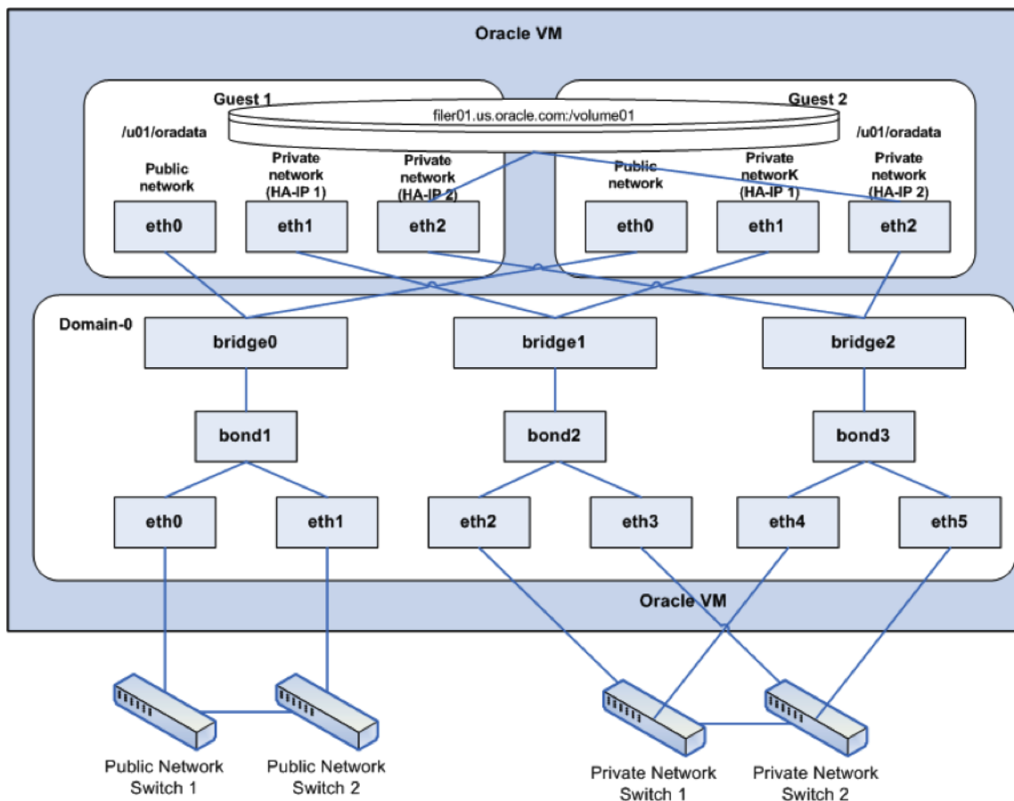
Figure 14: Full network bonding on Oracle Linux KVM
