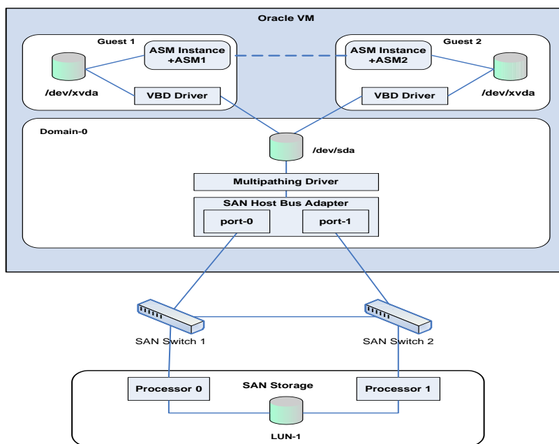
Figure 13: SAN storage on Oracle Linux KVM
