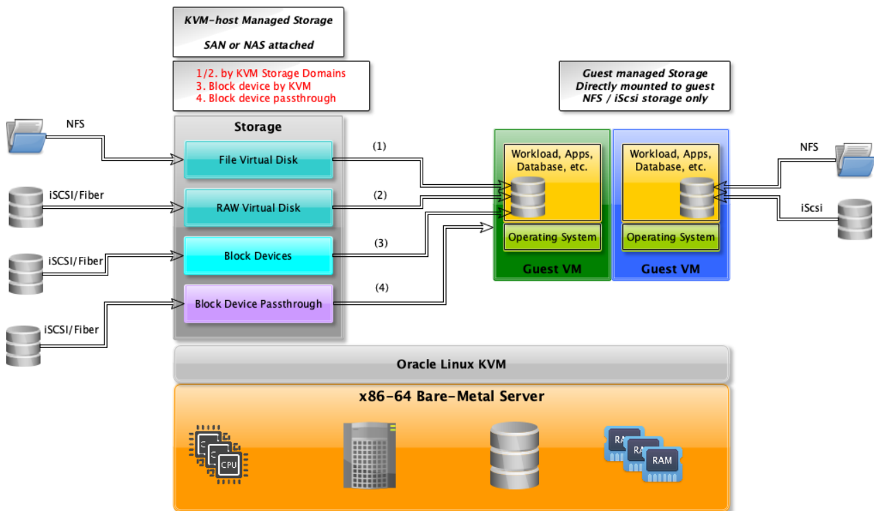
Figure 12: Storage configuration options on Oracle Linux KVM
