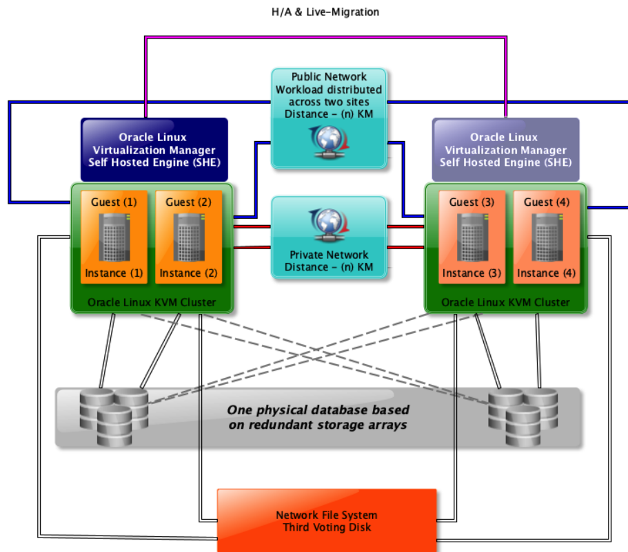
Figure 8: Oracle Extended RAC on Oracle Linux KVM – Single Oracle Linux Virtualization Manager
