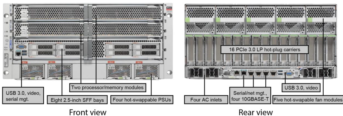
Figure 11. SPARC T7-4 server front and rear perspectives.
