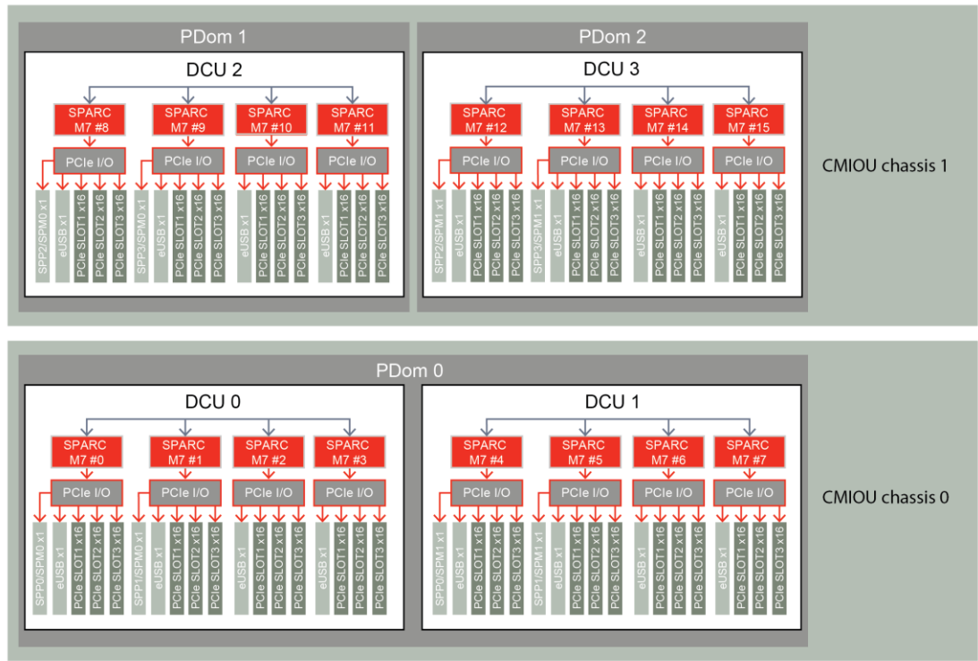
Figure 22. The SPARC M7-16 server is divided into four domain configurable units (DCUs) which can be flexibly combined to create one, two, three, or four PDom (three PDom shown).
