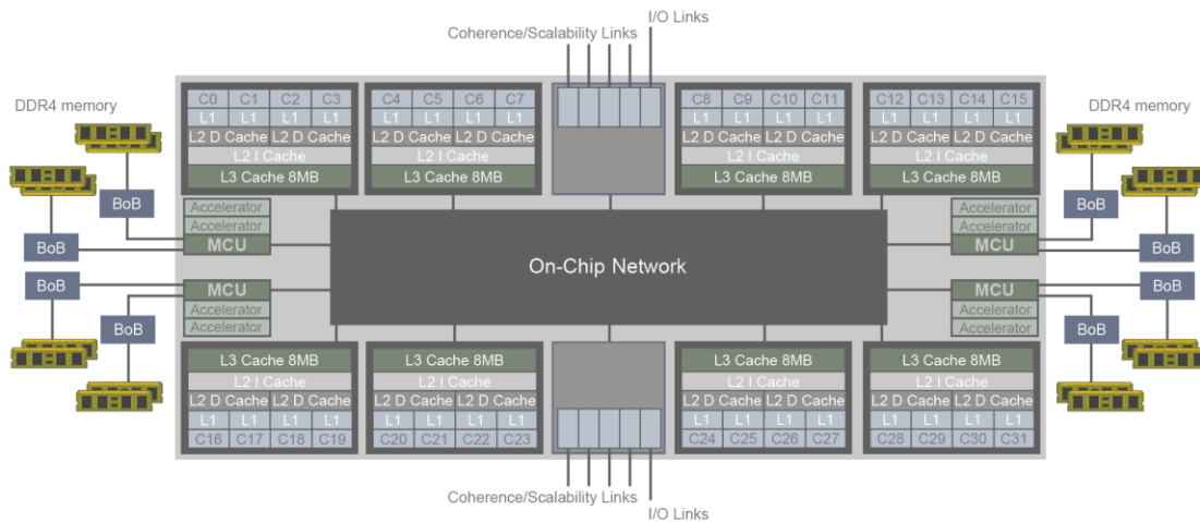
Figure 3. The SPARC M7 processor features 32 cores, eight SPARC core clusters, four memory controller units (MCUs), and eight Data Analytics Accelerators (DAXs).
