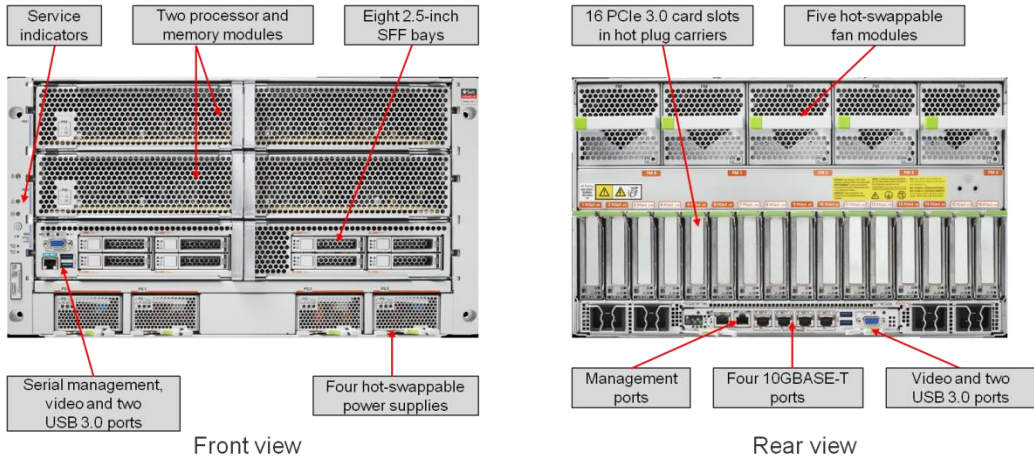
Figure 11. SPARC T8-4 server front and rear perspectives.
