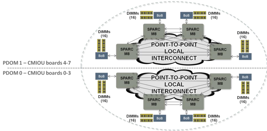
Figure 19. The SPARC M8-8 server with two PDOMs is composed of two all-to-all interconnects.
