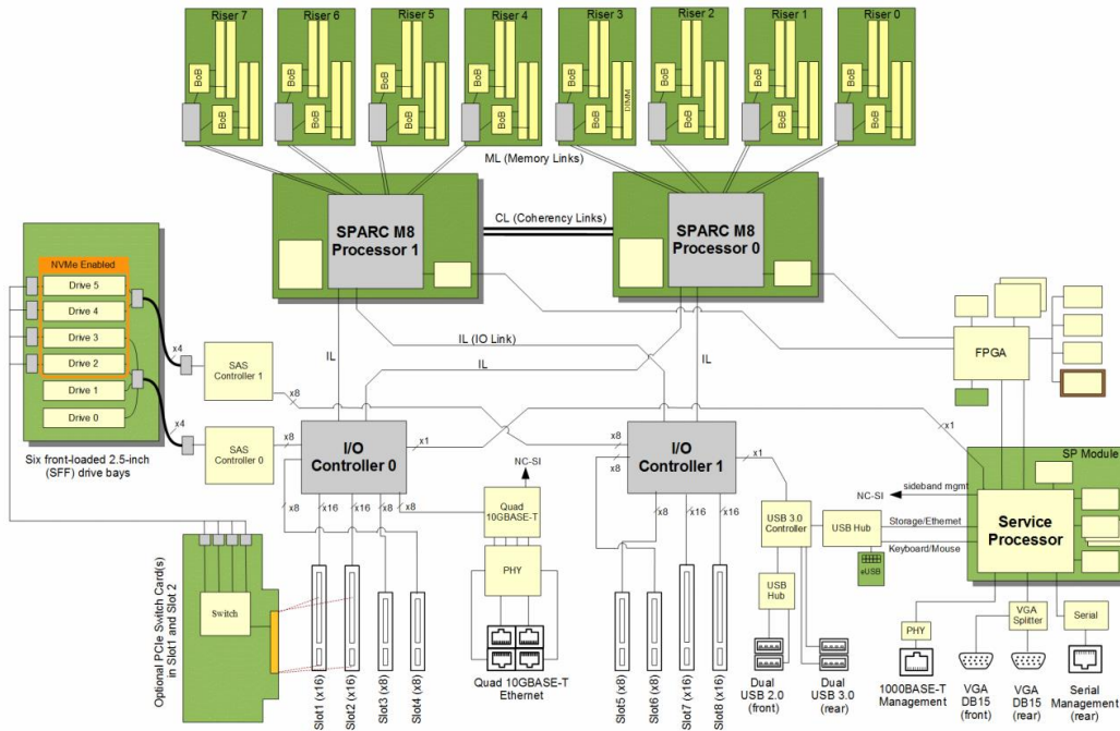
Figure 10. The SPARC T8-2 server has dual SPARC M8 processors cross-connected to two I/O controller ASICs for higher availability.
