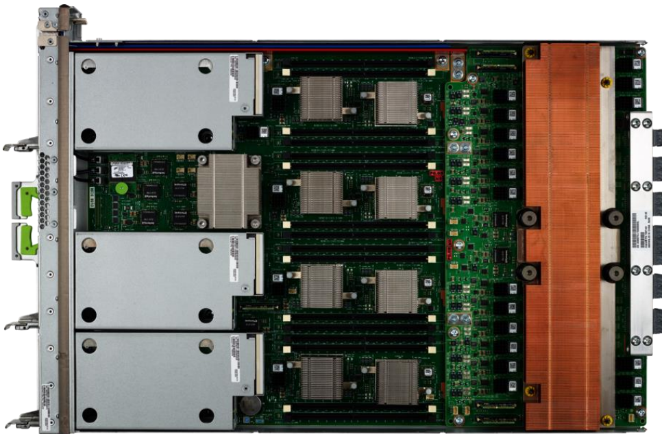
Figure 15. Each CMIU board contains a SPARC M8 processor, 16 DDR4 DIMM slots, an I/O controller ASIC, and three PCIe x16 hot-pluggable carriers.
