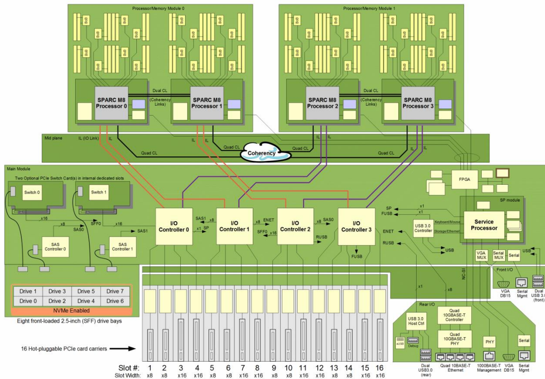
Figure 12. SPARC T8-4 servers feature two dual-processor/memory modules and four I/O controllers ASICs.
