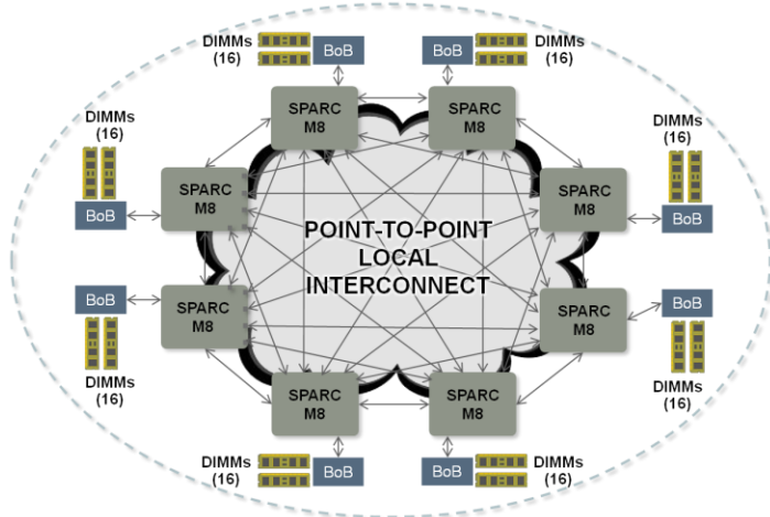
Figure 17. The eight-way all-to-all interconnect of the SPARC M8-8 server.
