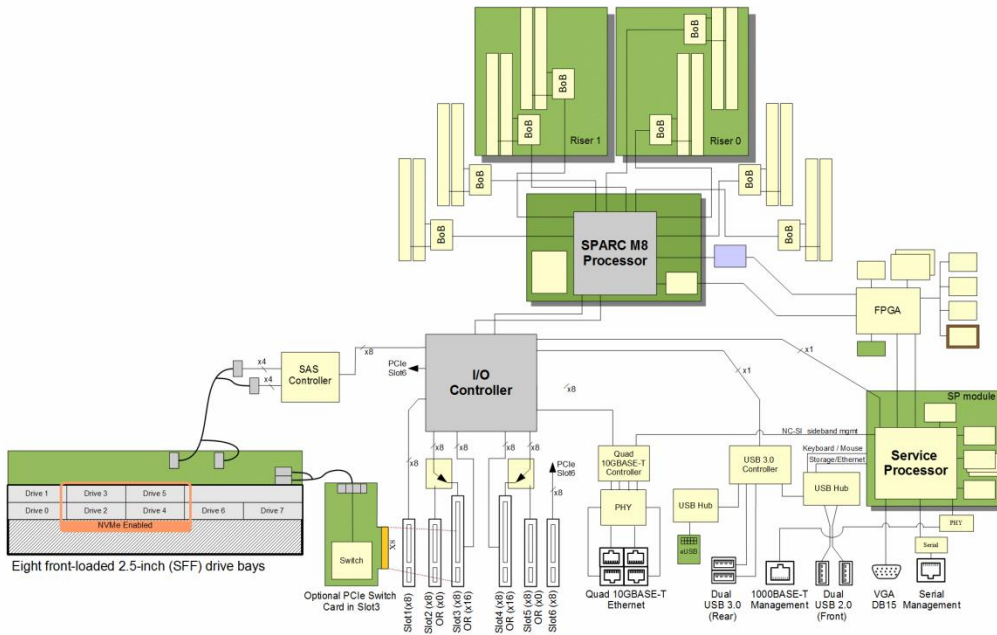
Figure 8. The SPARC T8-1 server features a single 32-core SPARC M8 processor and I/O controller ASIC.
