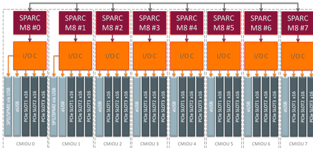
Figure 16. This SPARC M8-8 server includes up to eight SPARC M8 processors and is factory-configured with a single PDom.
