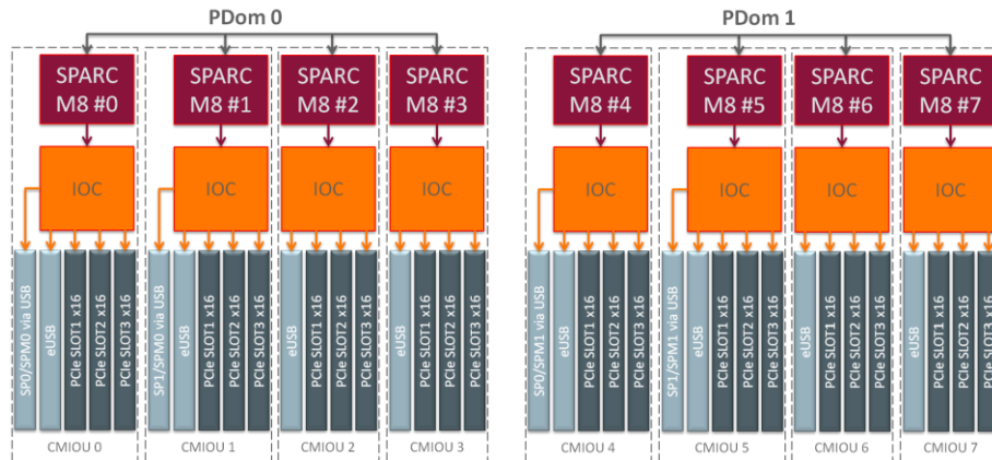
Figure 18. The SPARC M8-8 server can be ordered factory-configured with two electrically isolated PDOMs.
