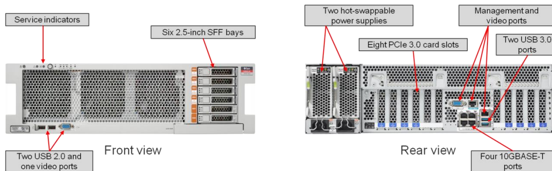
Figure 9. SPARC T8-2 server front and rear perspectives.
