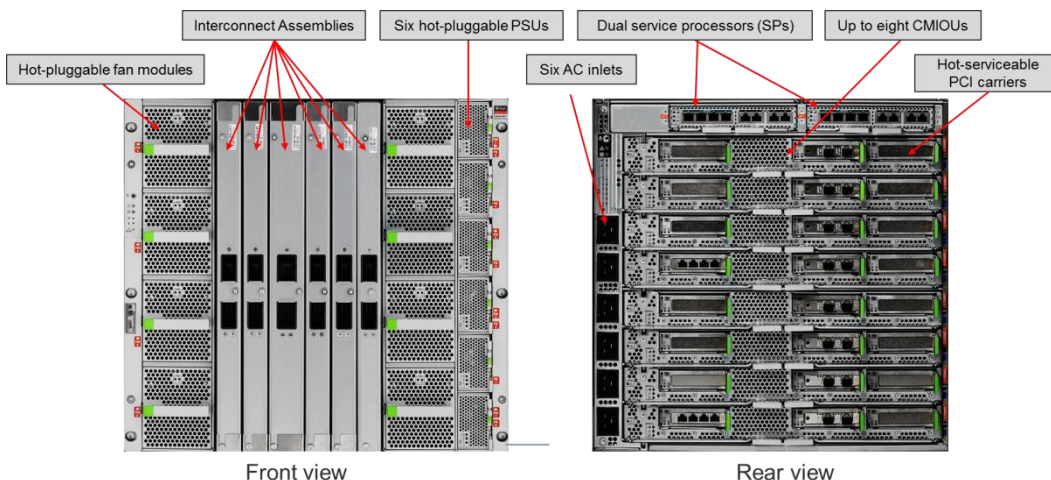
Figure 13. Front and rear perspectives of the SPARC M8-8 CMIOU chassis.
