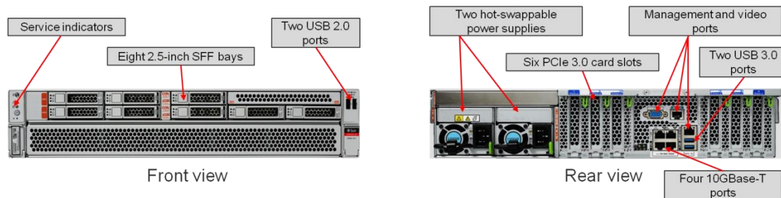
Figure 7. SPARC T8-1 server front and rear perspectives.
