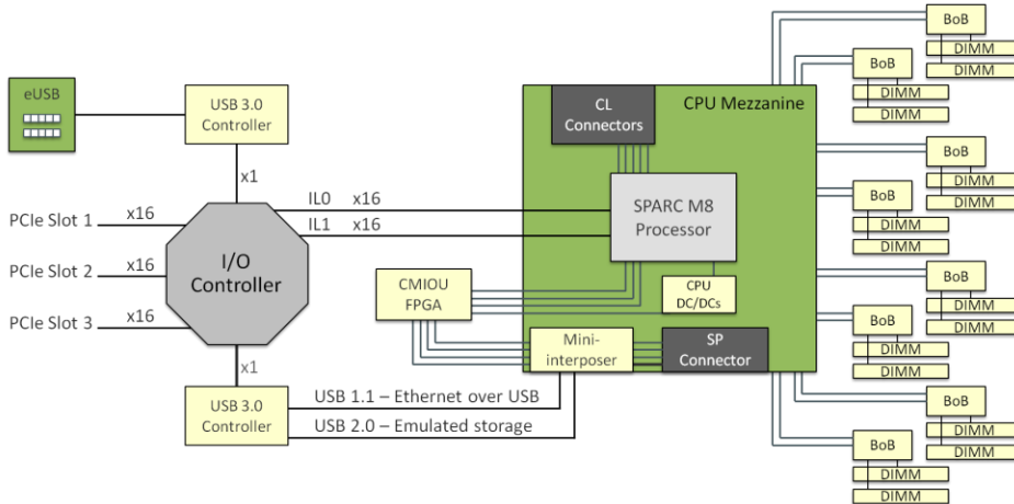
Figure 14. Architectural perspective of a single SPARC M8-8 CMIU board.
