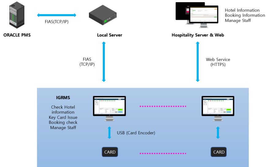
High-level architecture of the integration between ImGATE and Oracle Hospitality OPERA.
