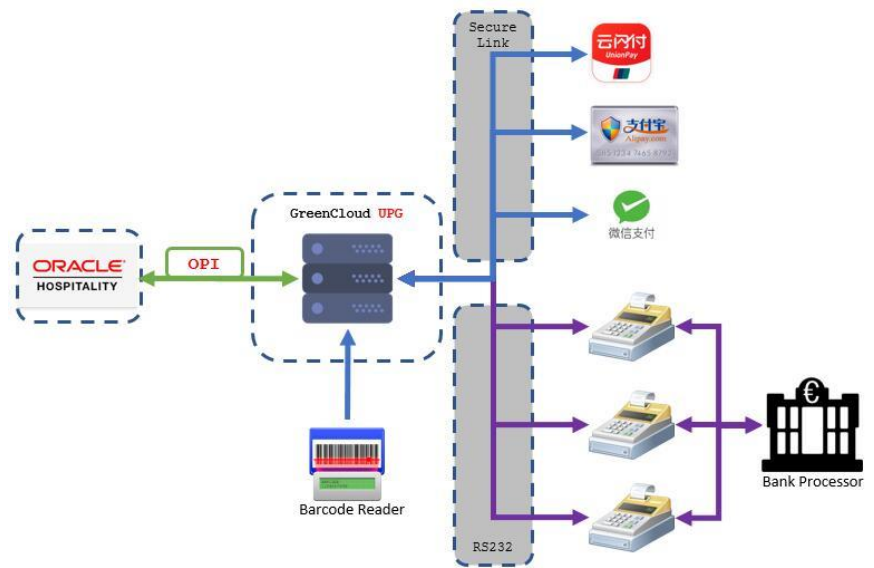
Figure 1. Integration architecture between Greencloud UPG and Oracle Payment Interface
