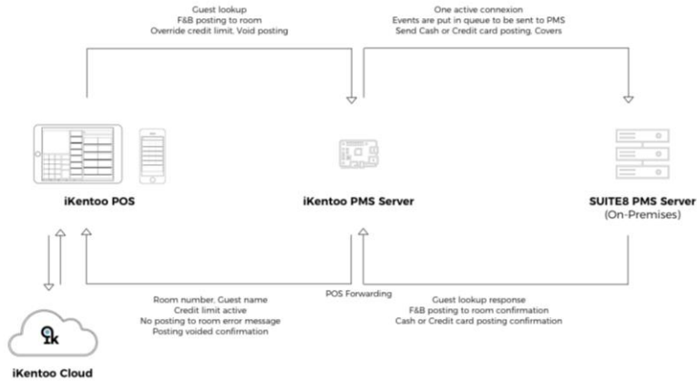
Figure 1. Integration diagram for iKentoo and Oracle Hospitality Suite8
