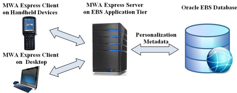
Figure. Architecture diagram for MWA Express Suite integration with Oracle E-Business Suite
