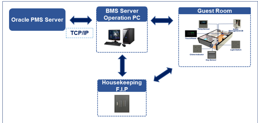
Figure 1. RACOS BMS system diagram
