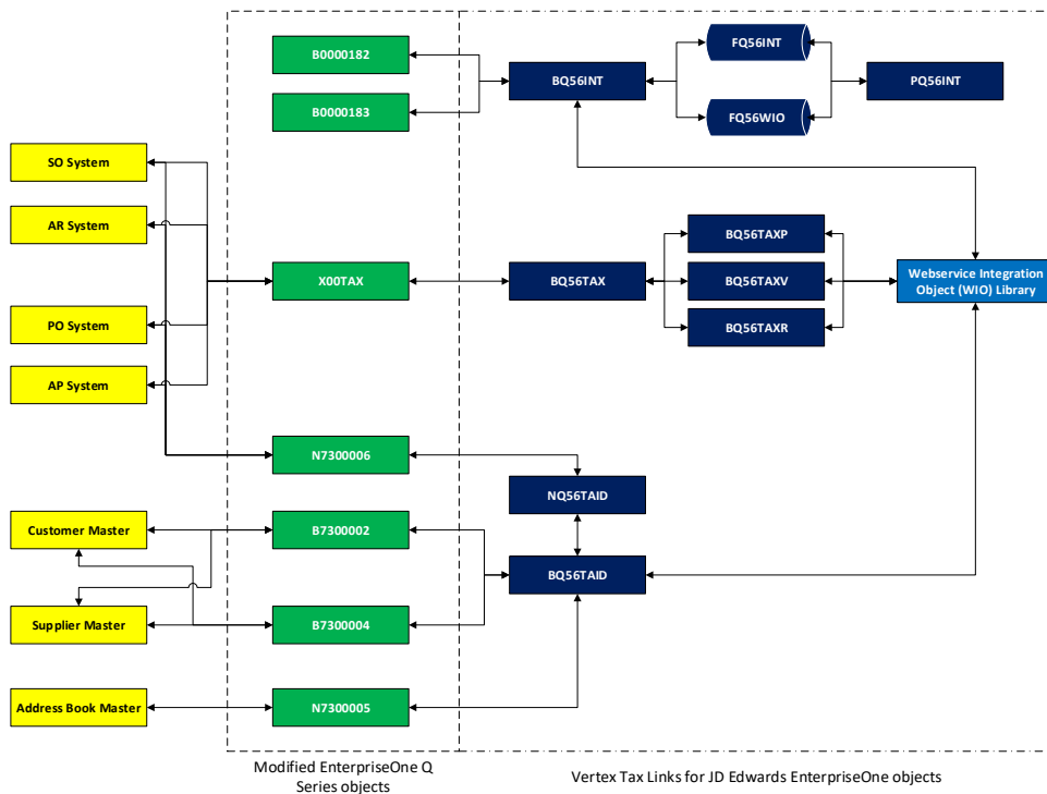
Architecture diagram for the validated integration between Vertex® Tax Links and JD Edwards EnterpriseOne
