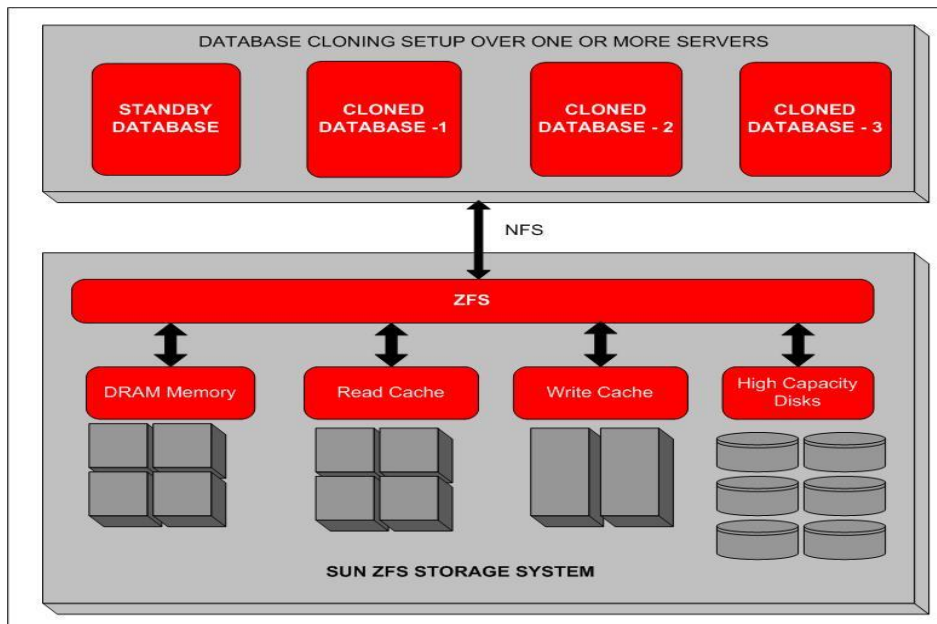
Figure 4. Sun ZFS Storage Appliance Hybrid Storage Pool used for database cloning.
