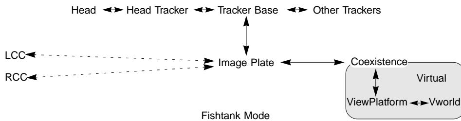
Figure C-1 Display Rigidly Attached to the Tracker Base
