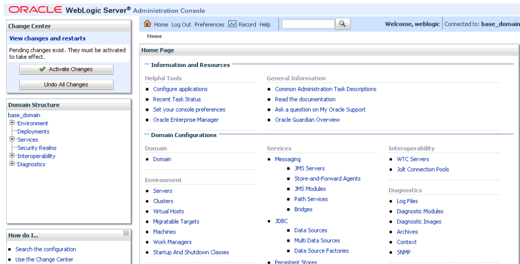
Figure 2-25 Oracle WebLogic Server Administration Console Home Page
