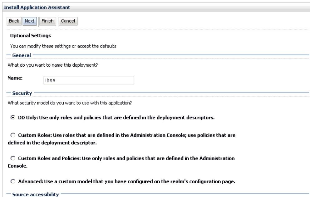
Figure 2–43 Optional Settings Page
