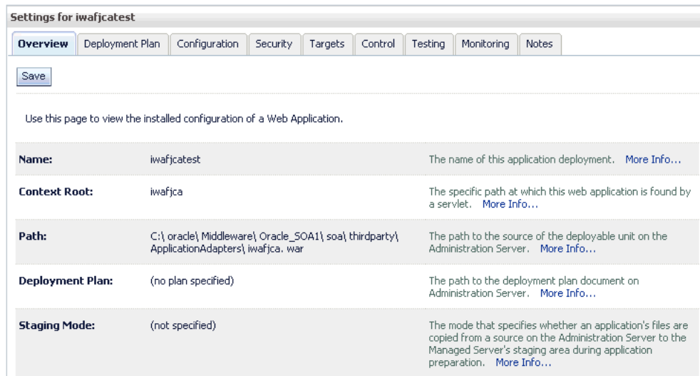
Figure 2–32 J2CA Settings Page
