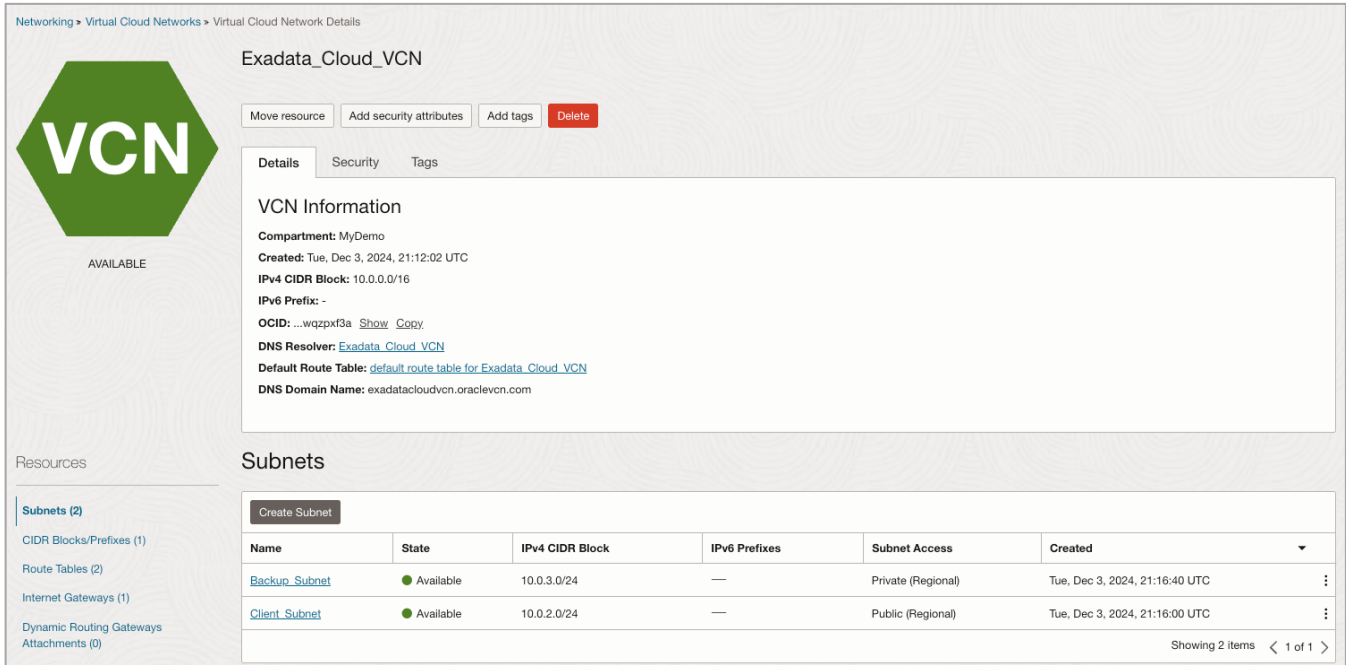
Figure 1: Oracle Cloud Infrastructure Virtual Cloud Network (VCN) Details
